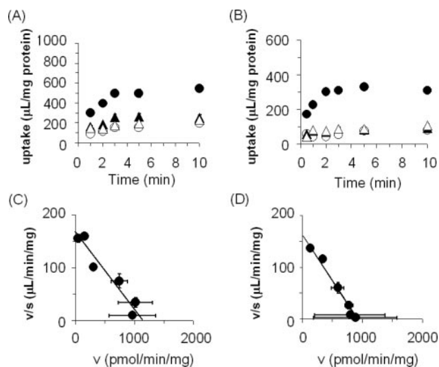
Fig. 1. Time profiles and Eadie-Hofstee plots of the uptake of [ ^3 H]pitavastatin by human and mouse BCRP-expressing membrane vesicles. The uptake of 0.1 \mu M [ ^3 H]pitavastatin by human BCRP (hBCRP) (A) and mouse Bcrp (mBcrp) (B), respectively, was examined at 37°C in medium containing 5 mM ATP (closed symbols) or AMP (open symbols). Circles and triangles represent the uptake in hBCRP- (or mBcrp-) and GFP-expressing membrane vesicles, respectively. The hBCRP- (C) and mBcrp- (D)-mediated uptake of [ ^3 H]pitavastatin was determined for 2 and 1 min, respectively. Each point represents the mean \pm S.E. ( n = 3 ). Where vertical bars are not shown, the S.E. values are within the limits of the symbols. The data were fitted to the Michaelis-Menten equation by non-linear regression analysis, as described under Materials and Methods , and each solid line represents the fitted curve.
